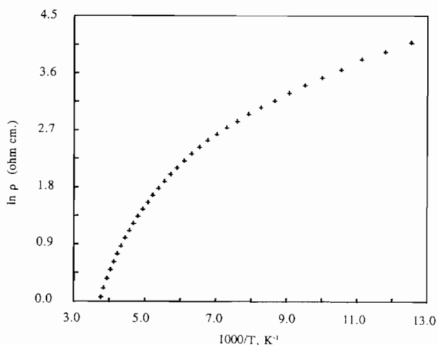
Fig. 1. A plot of \ln \rho vs. 1000/T ( T in units of K) for (\text{TTF})_5\text{Fe}(\text{NO}_3)_3 .
